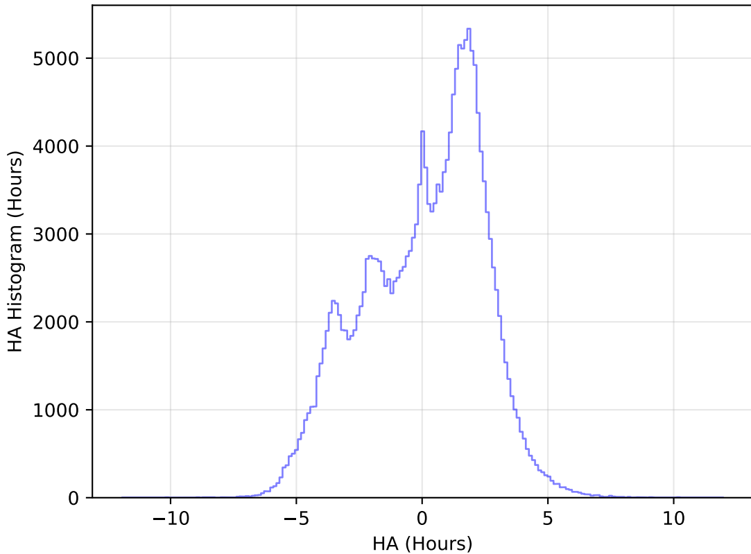
weather_cloudso35v3.4_10yrs WFD g band: HA Histogram
