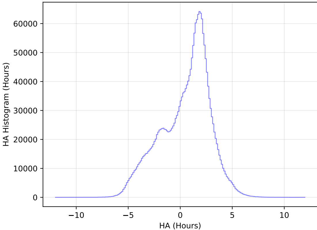
weather_cloudso35v3.4_10yrs WFD all bands: HA Histogram
