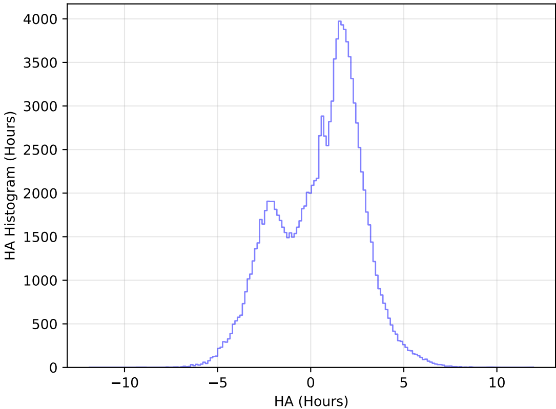
weather_cloudso35v3.4_10yrs All sky u band: HA Histogram
