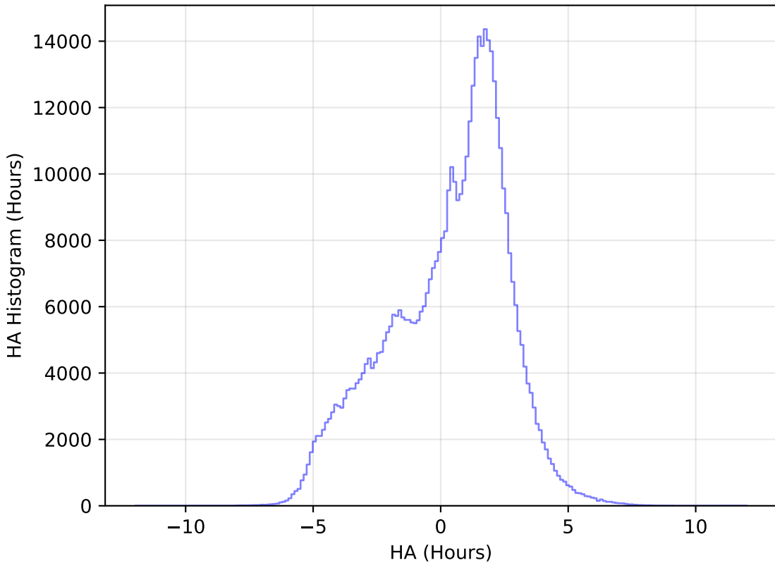
weather_cloudso35v3.4_10yrs All sky r band: HA Histogram
