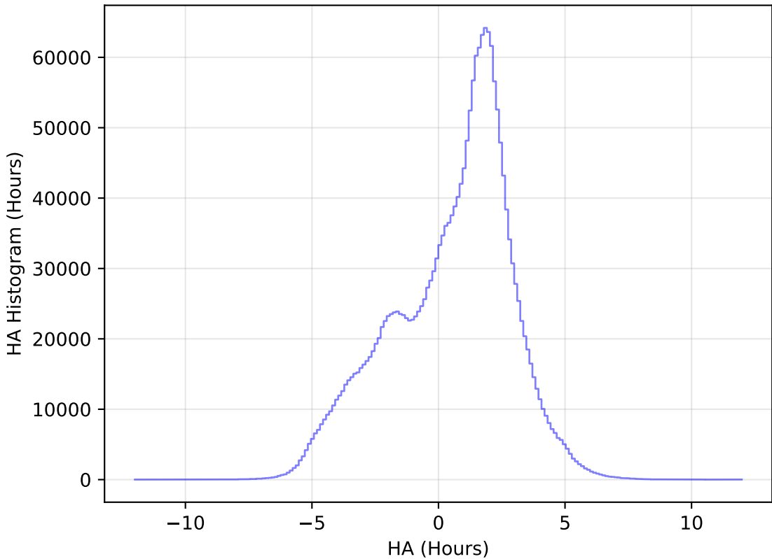
weather_cloudso35v3.4_10yrs All sky all bands: HA Histogram
