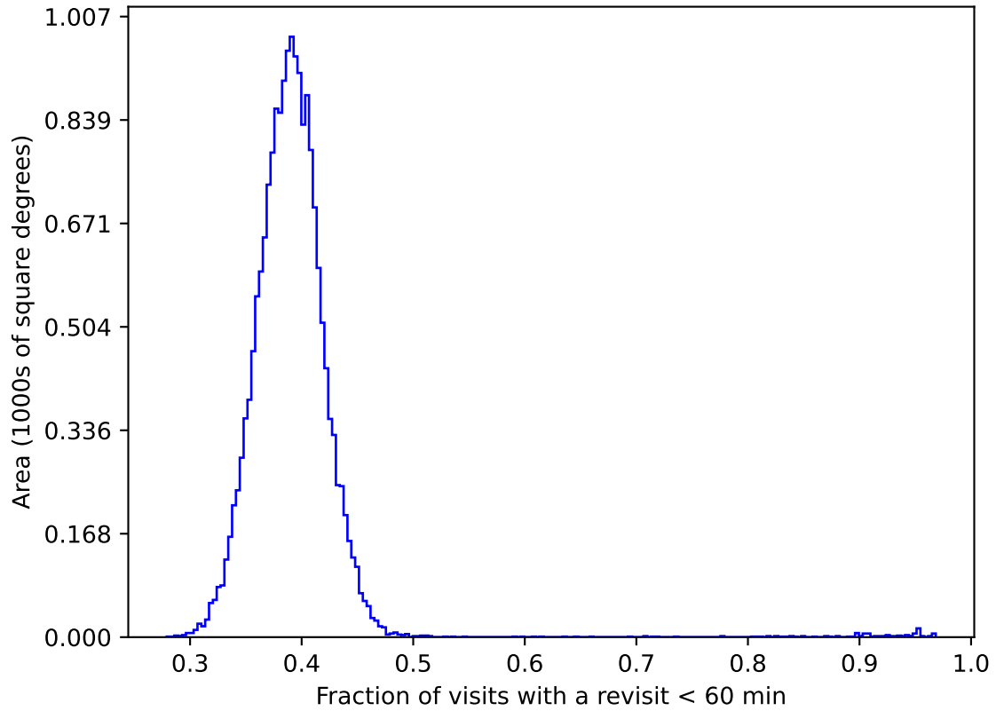
weather_cloudso35v3.4_10yrs gri WFD: Fraction of visits with a revisit < 60 min
