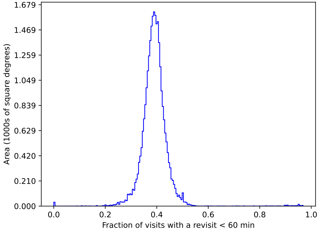
weather_cloudso35v3.4_10yrs gri All sky: Fraction of visits with a revisit < 60 min
