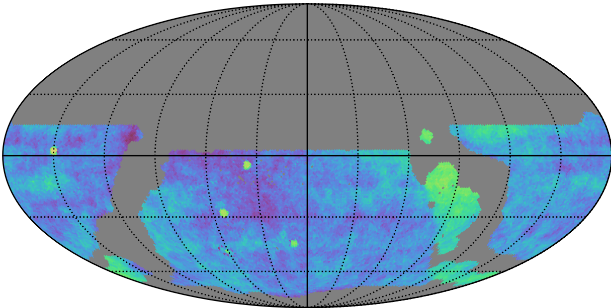
weather_cloudso35v3.4_10yrs gri WFD: Fraction of visits in pairs (20-90 min)
