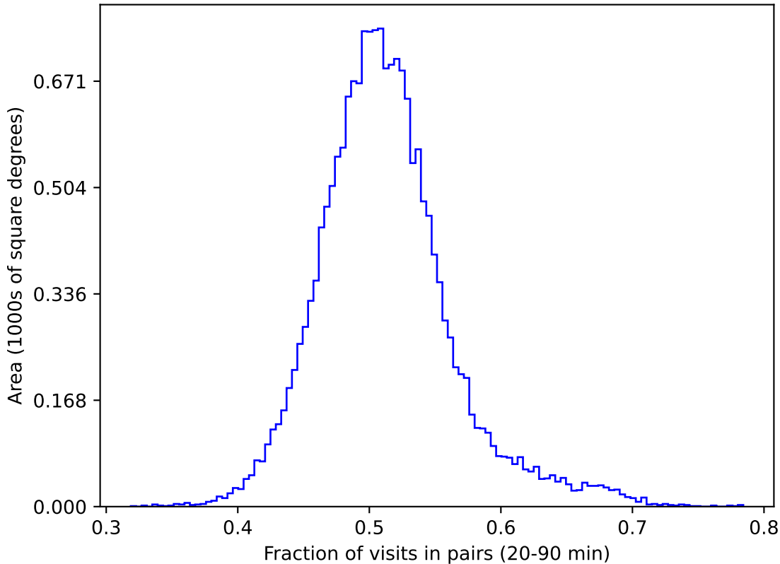
weather_cloudso35v3.4_10yrs gri WFD: Fraction of visits in pairs (20-90 min)
