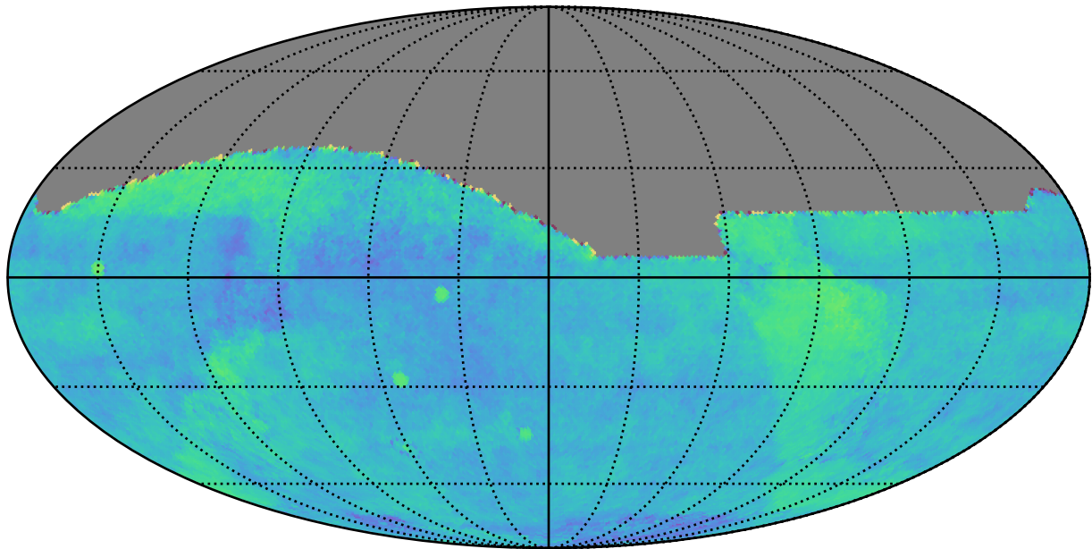
weather_cloudso35v3.4_10yrs gri All sky: Fraction of visits in pairs (20-90 min)
