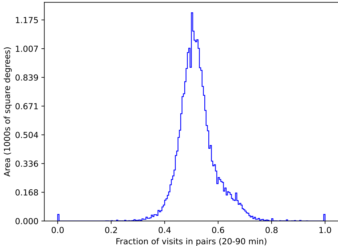
weather_cloudso35v3.4_10yrs gri All sky: Fraction of visits in pairs (20-90 min)
