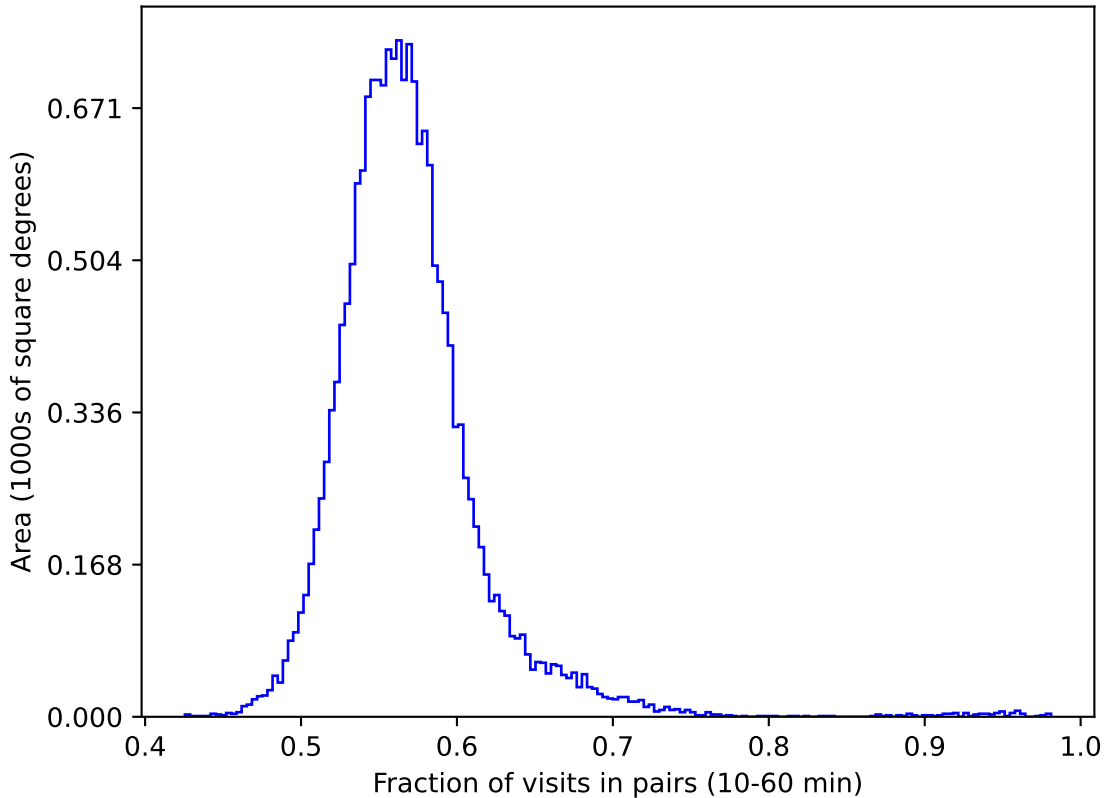
weather_cloudso35v3.4_10yrs gri WFD: Fraction of visits in pairs (10-60 min)
