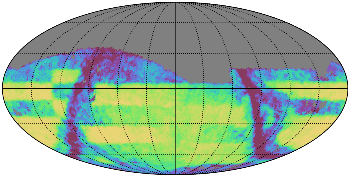
weather_cloudso35v3.4_10yrs Yr 3-4 z band: Exgal_CoaddM5
