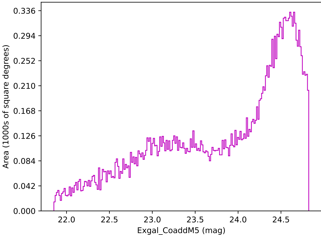
weather_cloudso35v3.4_10yrs Yr 3-4 z band: Exgal_CoaddM5
