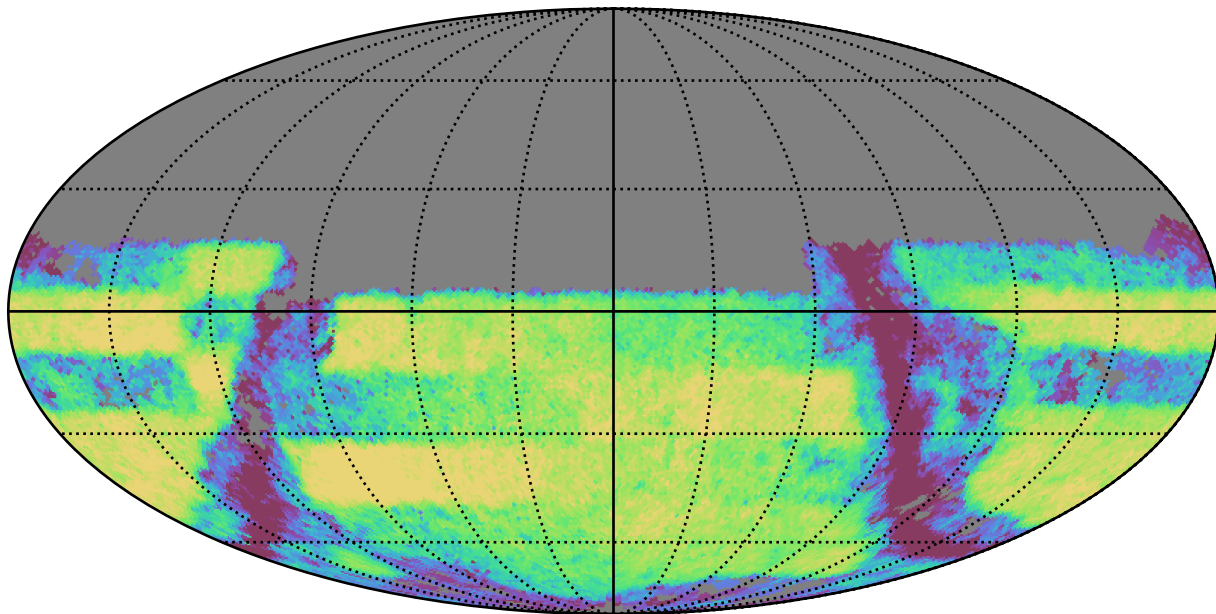
weather_cloudso35v3.4_10yrs Yr 3-4 y band: Exgal_CoaddM5
