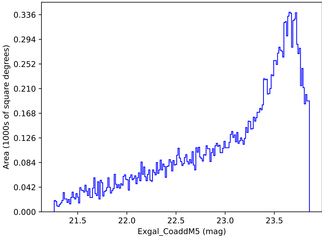
weather_cloudso35v3.4_10yrs Yr 3-4 y band: Exgal_CoaddM5
