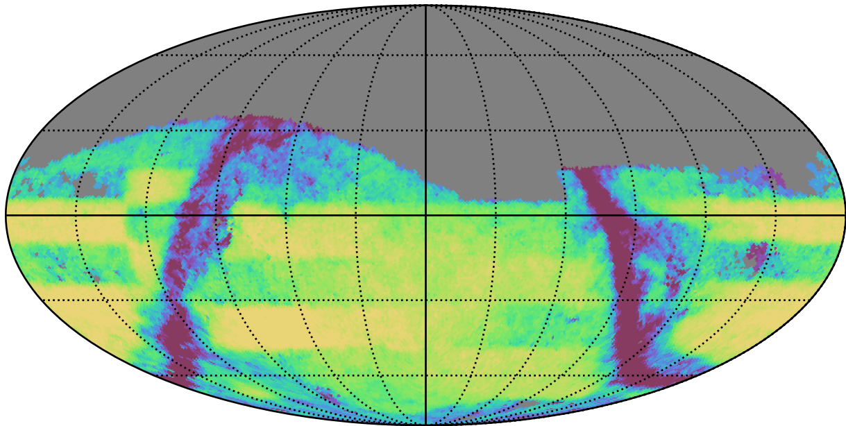
weather_cloudso35v3.4_10yrs Yr 3-4 r band: Exgal_CoaddM5
