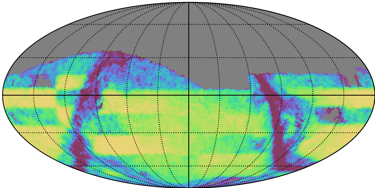
weather_cloudso35v3.4_10yrs Yr 3-4 i band: Exgal_CoaddM5
