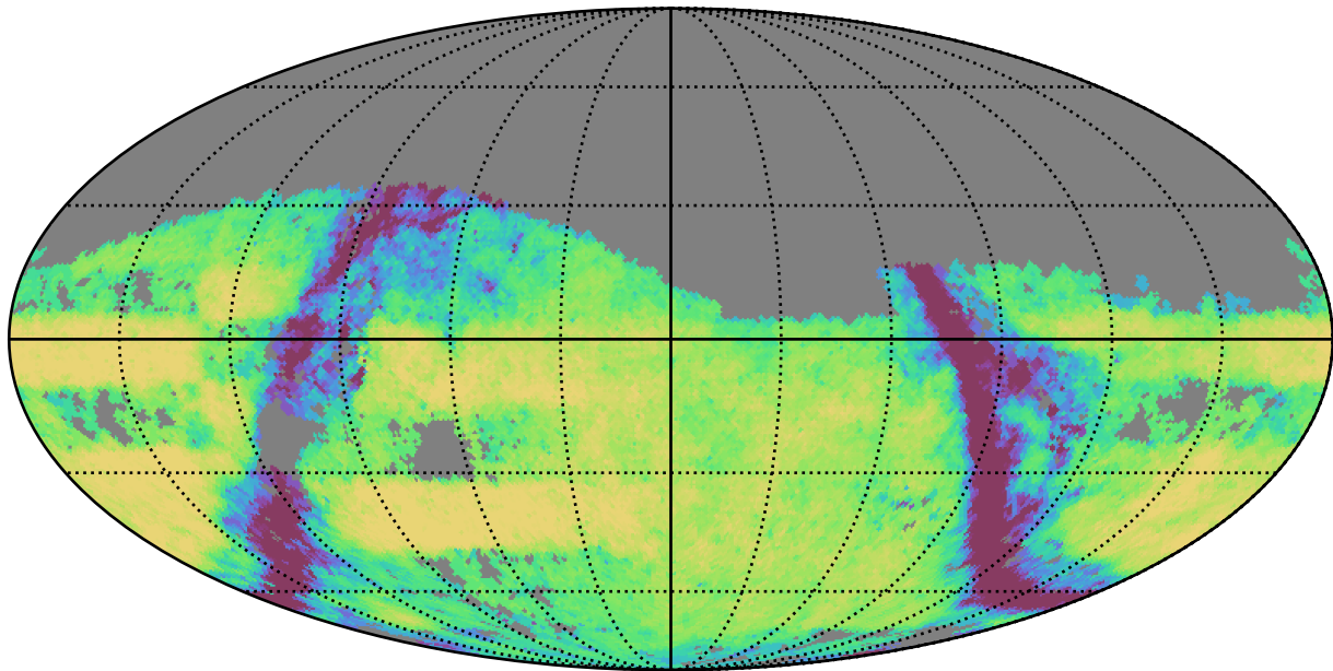
weather_cloudso35v3.4_10yrs Yr 3-4 g band: Exgal_CoaddM5
