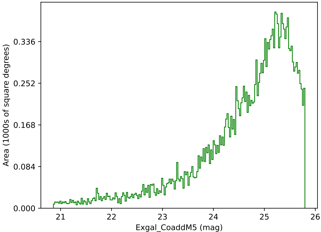
weather_cloudso35v3.4_10yrs Yr 3-4 g band: Exgal_CoaddM5
