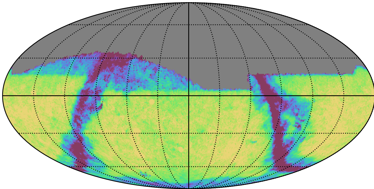
weather_cloudso35v3.4_10yrs Yr 1 z band: Exgal_CoaddM5
