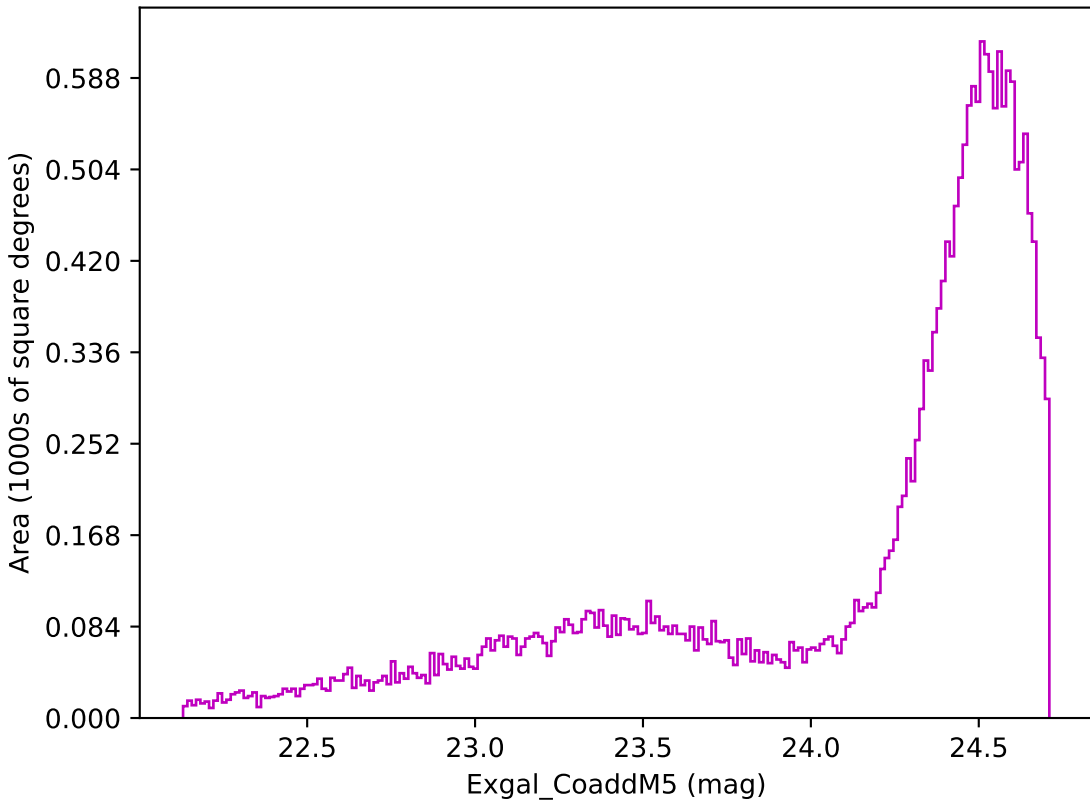
weather_cloudso35v3.4_10yrs Yr 1 z band: Exgal_CoaddM5
