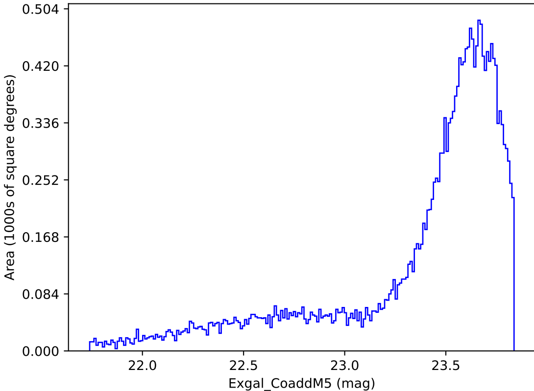
weather_cloudso35v3.4_10yrs Yr 1 y band: Exgal_CoaddM5
