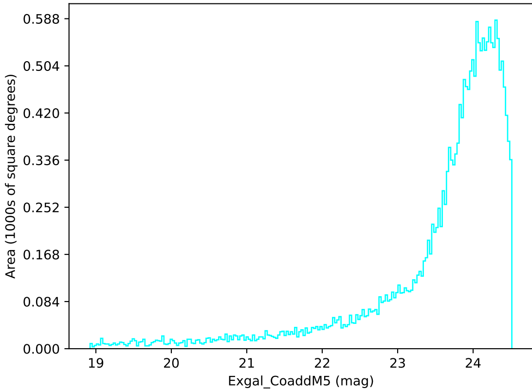
weather_cloudso35v3.4_10yrs Yr 1 u band: Exgal_CoaddM5
