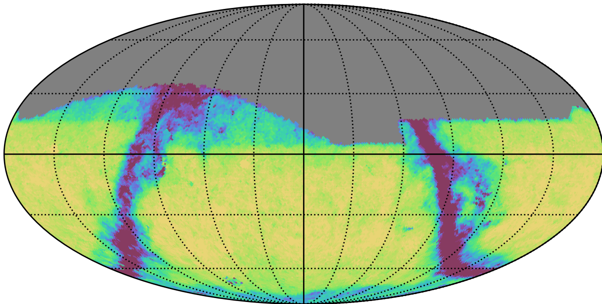
weather_cloudso35v3.4_10yrs Yr 1 r band: Exgal_CoaddM5
