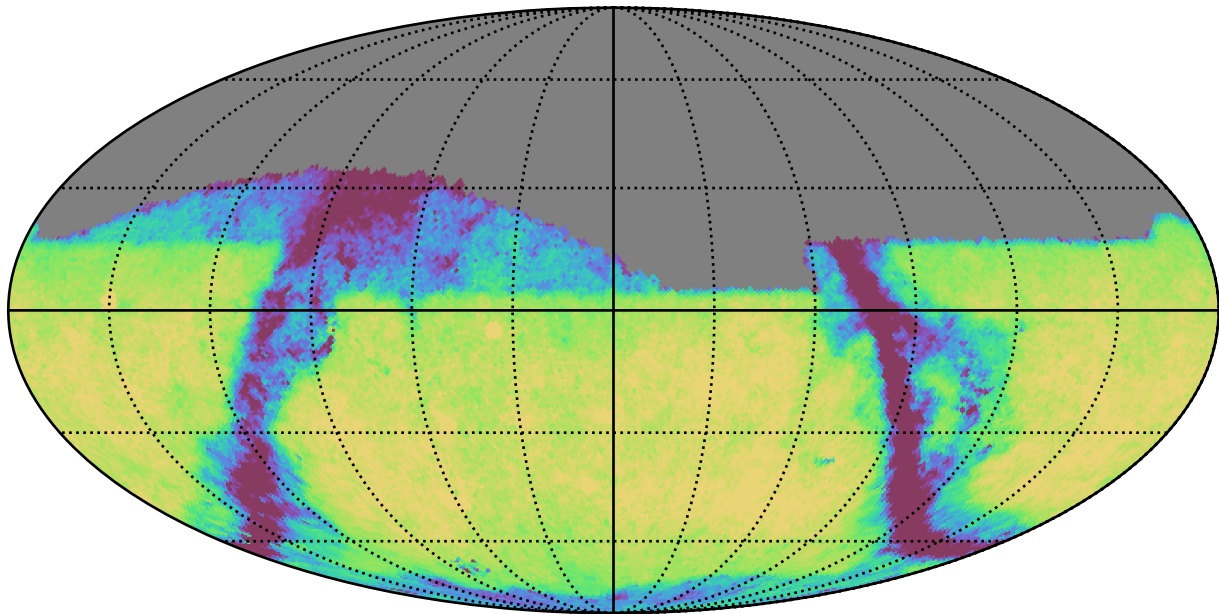
weather_cloudso35v3.4_10yrs Yr 1 i band: Exgal_CoaddM5
