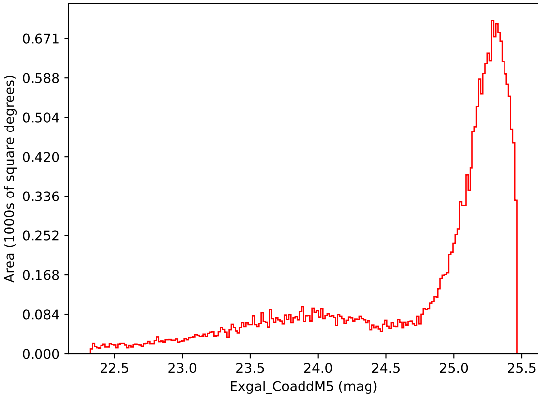
weather_cloudso35v3.4_10yrs Yr 1 i band: Exgal_CoaddM5
