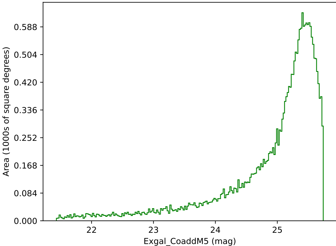
weather_cloudso35v3.4_10yrs Yr 1 g band: Exgal_CoaddM5
