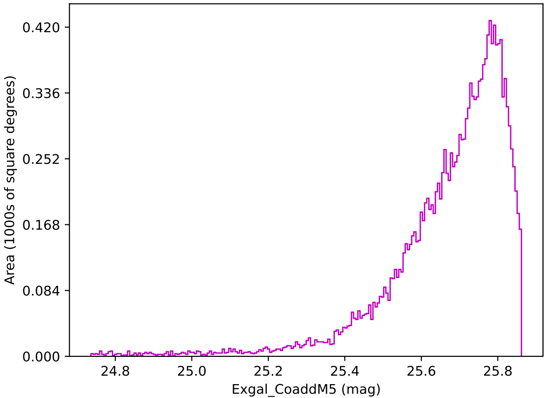
weather_cloudso35v3.4_10yrs WFD z band: Exgal_CoaddM5
