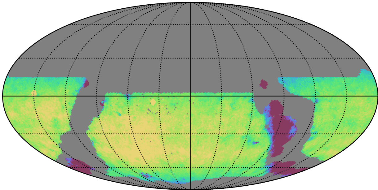
weather_cloudso35v3.4_10yrs WFD y band: Exgal_CoaddM5
