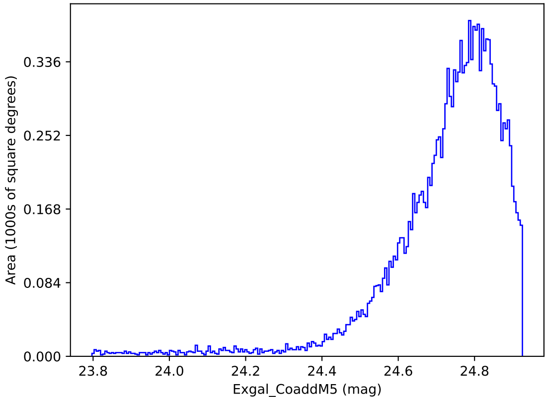
weather_cloudso35v3.4_10yrs WFD y band: Exgal_CoaddM5
