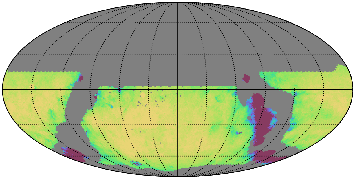
weather_cloudso35v3.4_10yrs WFD u band: Exgal_CoaddM5
