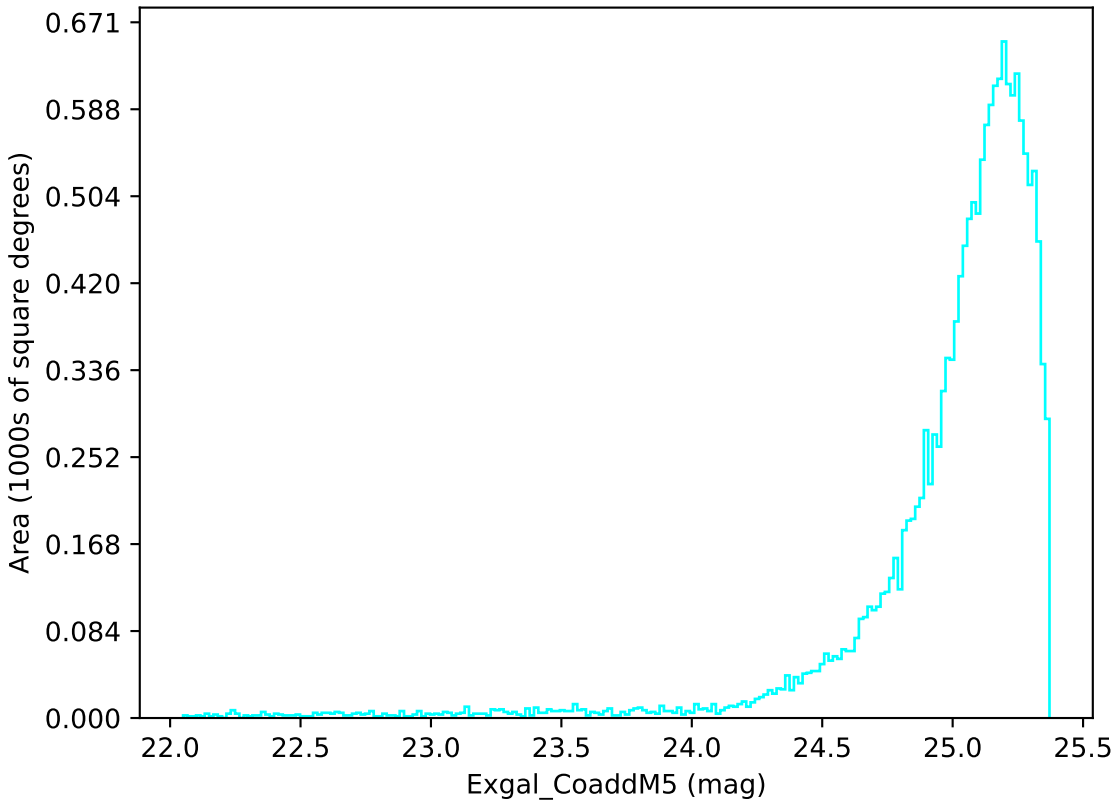
weather_cloudso35v3.4_10yrs WFD u band: Exgal_CoaddM5
