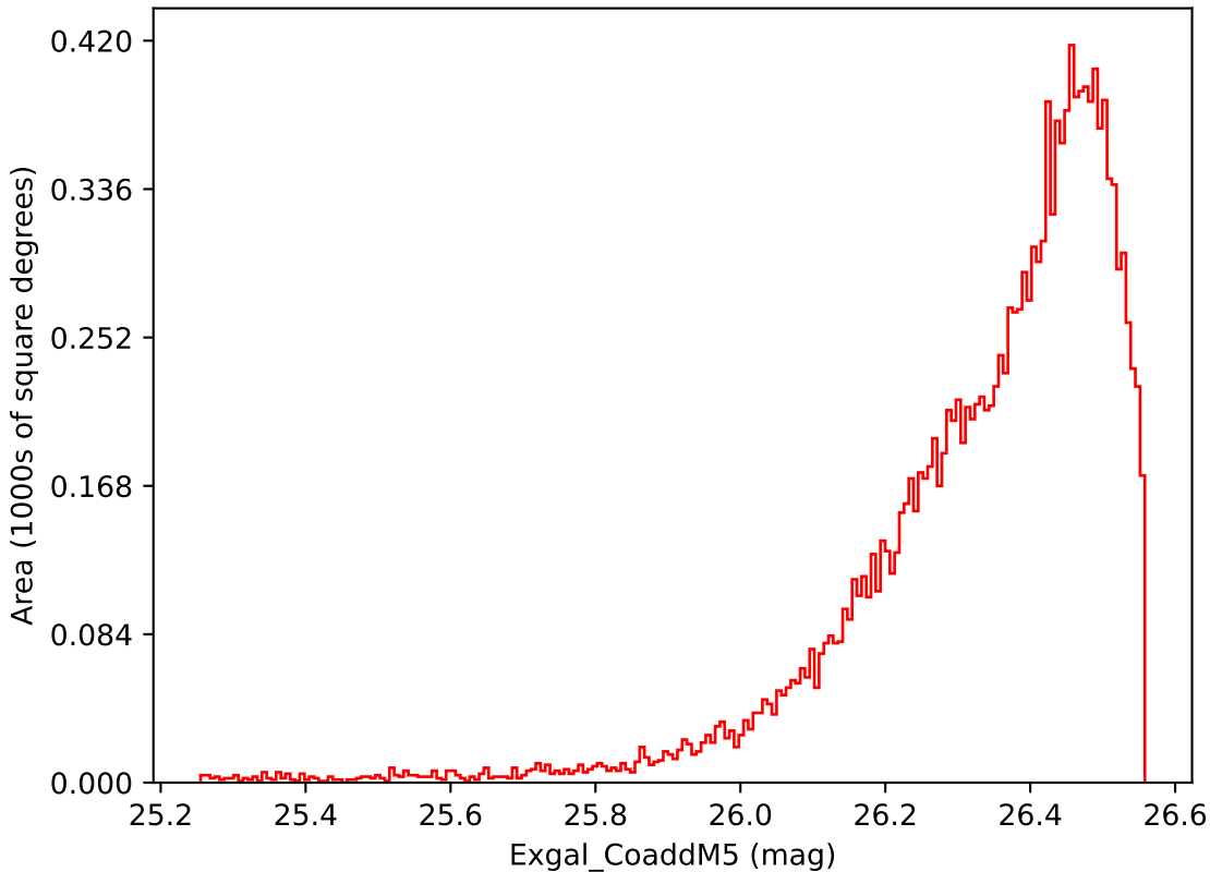
weather_cloudso35v3.4_10yrs WFD i band: Exgal_CoaddM5
