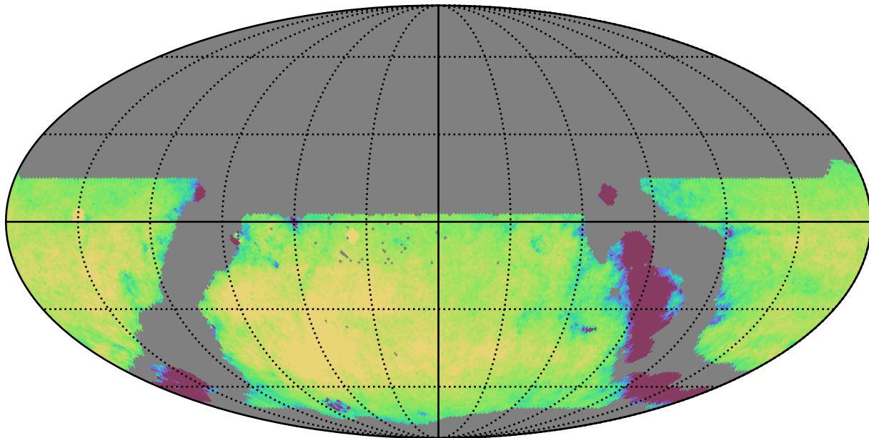
weather_cloudso35v3.4_10yrs WFD g band: Exgal_CoaddM5
