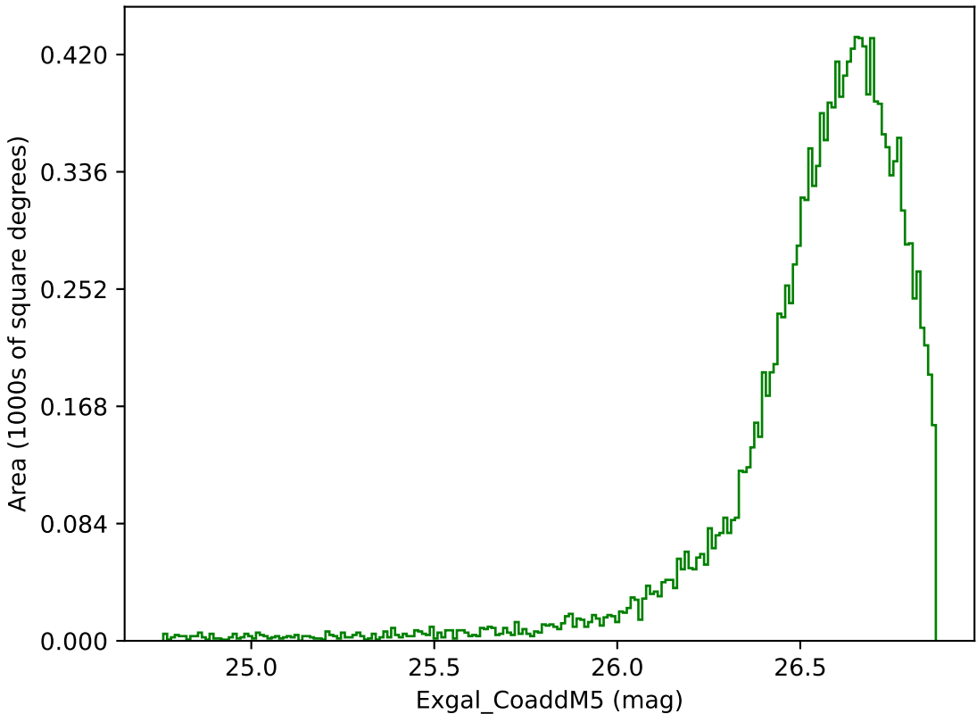
weather_cloudso35v3.4_10yrs WFD g band: Exgal_CoaddM5
