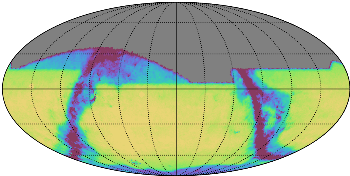
weather_cloudso35v3.4_10yrs All sky z band: Exgal_CoaddM5
