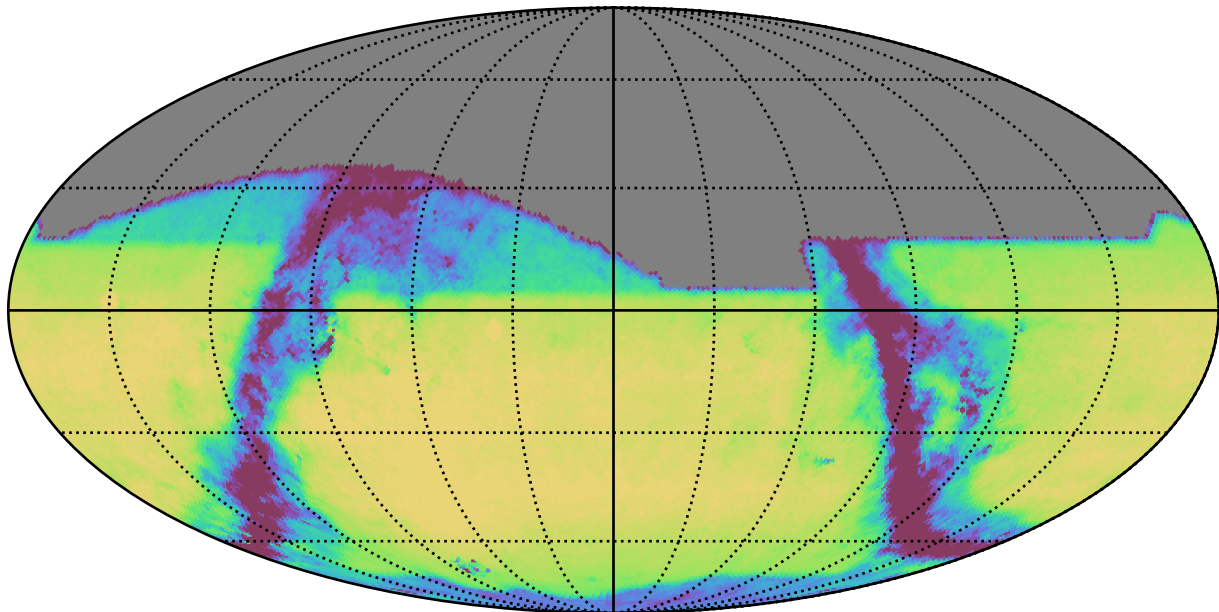
weather_cloudso35v3.4_10yrs All sky i band: Exgal_CoaddM5
