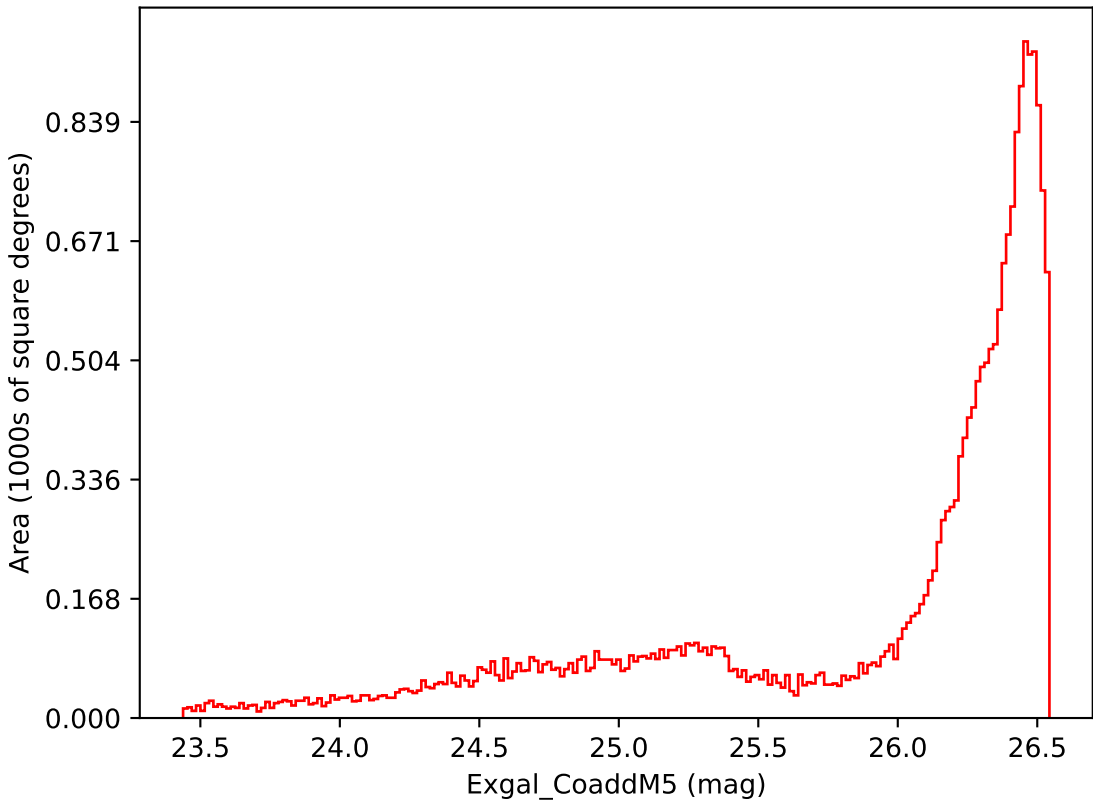
weather_cloudso35v3.4_10yrs All sky i band: Exgal_CoaddM5
