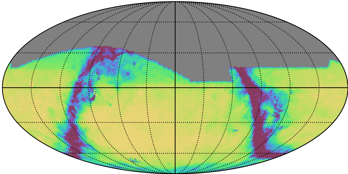
weather_cloudso35v3.4_10yrs All sky g band: Exgal_CoaddM5
