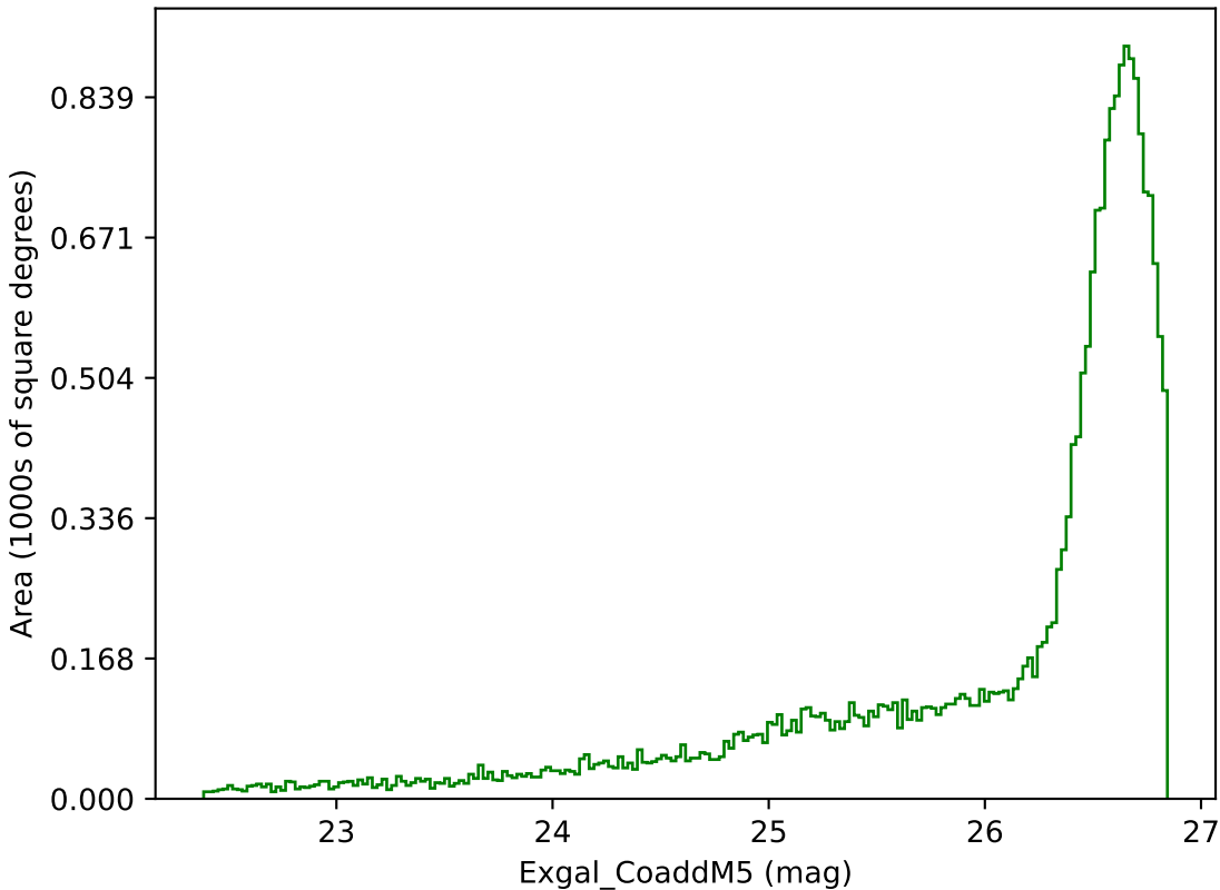
weather_cloudso35v3.4_10yrs All sky g band: Exgal_CoaddM5
