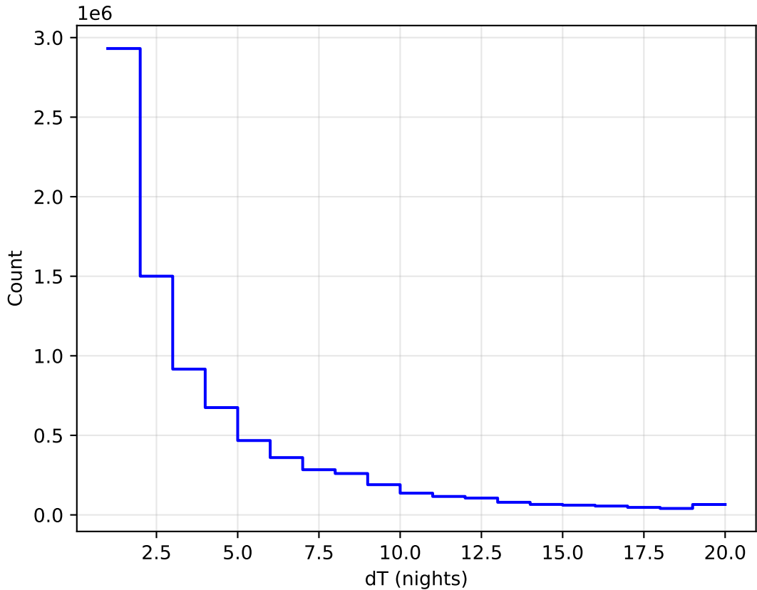
weather_cloudso35v3.4_10yrs WFD all bands: DeltaNight Histogram
