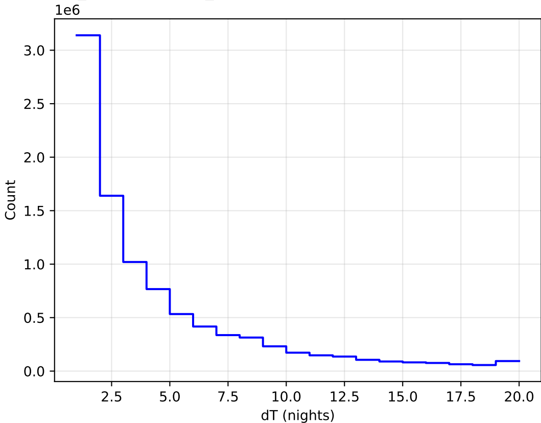
weather_cloudso35v3.4_10yrs All sky all bands: DeltaNight Histogram
