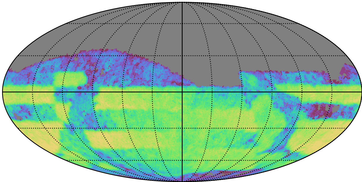
weather_cloudso35v3.4_10yrs Yr 3-4 z band: CoaddM5
