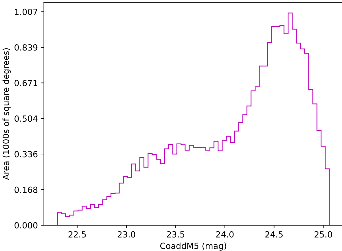
weather_cloudso35v3.4_10yrs Yr 3-4 z band: CoaddM5
