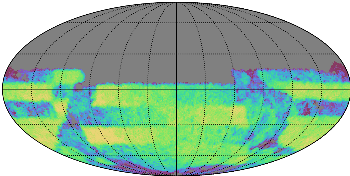
weather_cloudso35v3.4_10yrs Yr 3-4 y band: CoaddM5
