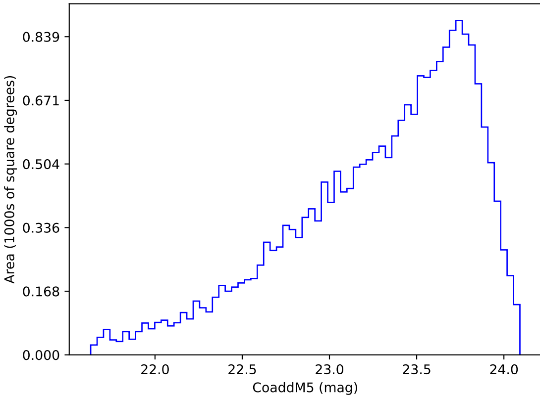
weather_cloudso35v3.4_10yrs Yr 3-4 y band: CoaddM5
