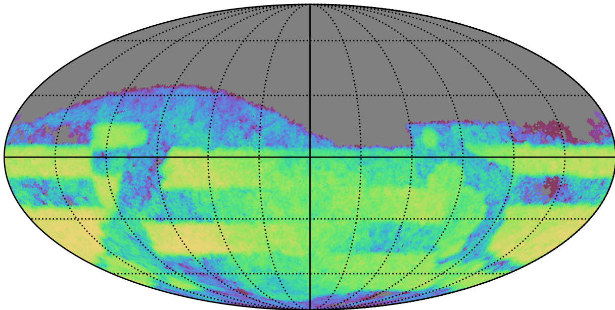
weather_cloudso35v3.4_10yrs Yr 3-4 r band: CoaddM5
