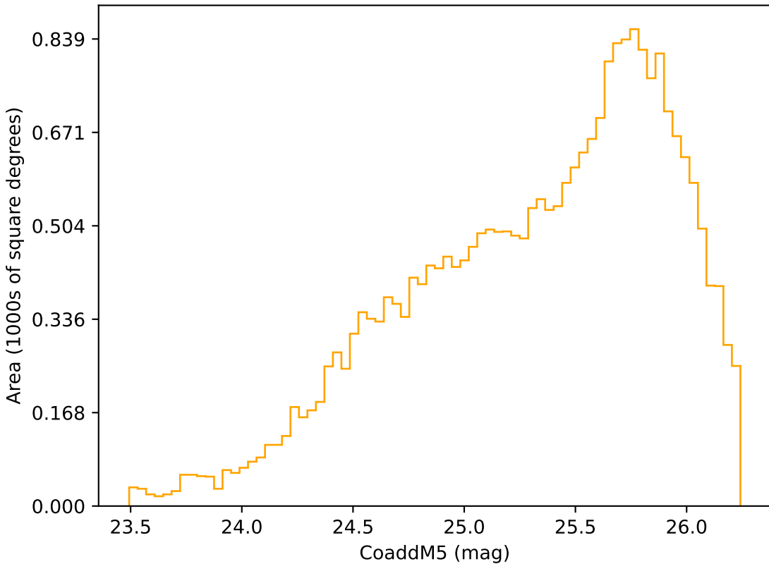
weather_cloudso35v3.4_10yrs Yr 3-4 r band: CoaddM5
