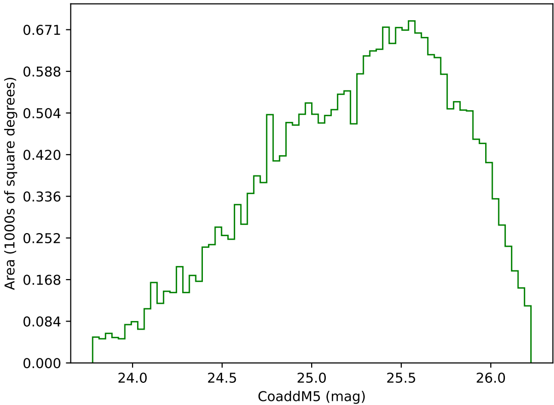
weather_cloudso35v3.4_10yrs Yr 3-4 g band: CoaddM5
